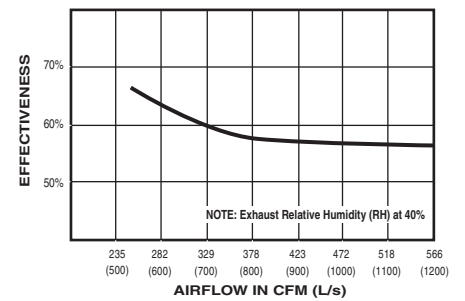
TEMPERATURE EFFECTIVENESS
