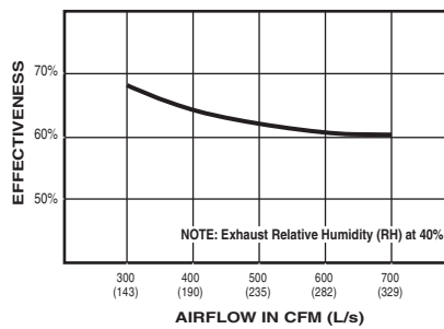
TEMPERATURE EFFECTIVENESS
